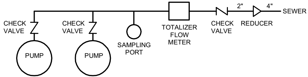
PUMP DETAIL
